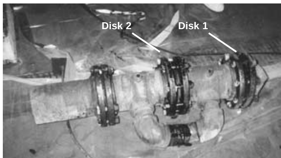
Figure 9: Rupture Disk Assembly Recovered from K-7 after the Incident (both disks blown)
