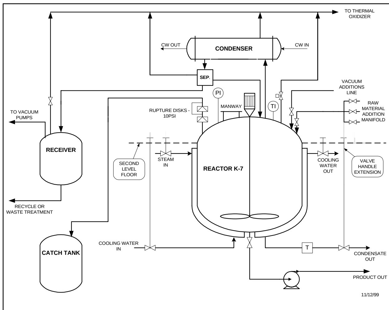
Figure 4: Simplified Process Flow Diagram
