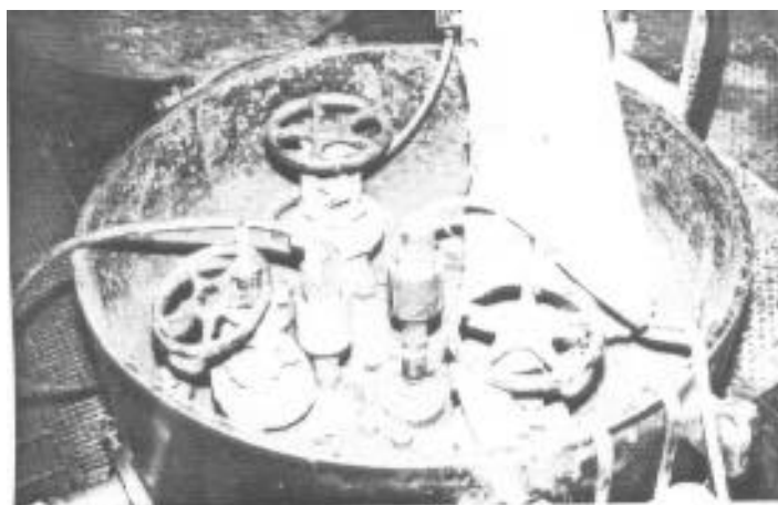
Tank car dome valving, showing level probes and insulated loading line to right rear angle valve.
